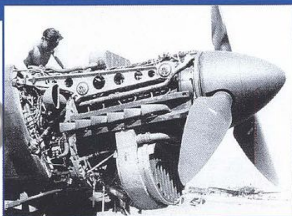
2690 JU-87 B2/STUKA COMPLETE ENGINE INSIDE
